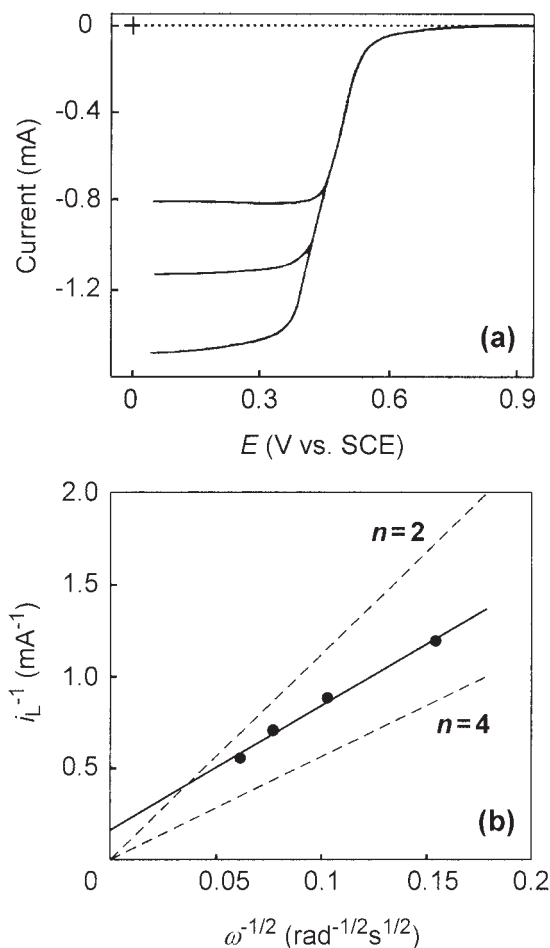
Fig. 2. (a) Current-potential curves for the reduction of O 2 obtained with the rotated glassy carbon electrode modified with the [Co(tp)(bim)] complex and the Pt/C catalyst. The active surface area of Pt/C was 5.58 cm 2 . The electrolyte solution was an O 2 -saturated aqueous HClO 4 (0.1 M). Electrode rotation rate was 400, 900, and 1600 rpm. Scan rate = 5 mV s -1 . (b) Koutecky-Levich plots of the plateau currents in (a) versus (electrode rotation rates) -1/2 . Dashed lines represent the diffusion limited currents for the two- ( n = 2 ) and four-electron ( n = 4 ) reduction of O 2 calculated using D = 2.9 \times 10^{-5} cm 2 s -1 , C = 1.3 \times 10^{-6} mol cm -3 , \nu (kinetic viscosity) = 0.01 cm 2 s -1 , and A = 0.28 cm 2 .
