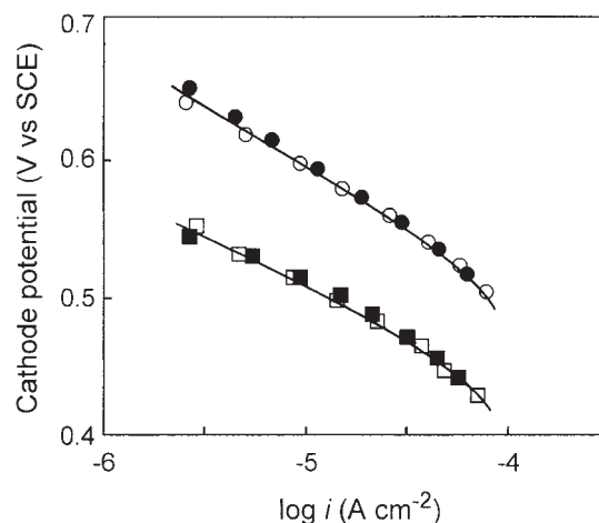
Fig. 3. Steady-state polarization curves for O 2 reduction on rotated modified electrodes recorded in an O 2 -saturated aqueous solution of HClO 4 (0.1 M). The electrode was a glassy carbon disk modified both with the [Co(tp)(bim)] complex and the Pt/C catalyst with the active surface area of 5.85 cm 2 (●), or the disk modified only with the Pt/C catalyst with the active surface area of 5.58 cm 2 (■). Open circles (○) and squares (□) represent plots of data obtained from repeated experiments using the same Pt/C-modified electrodes with and without the [Co(tp)(bim)] complex, respectively. Electrode rotation rate = 900 rpm.
