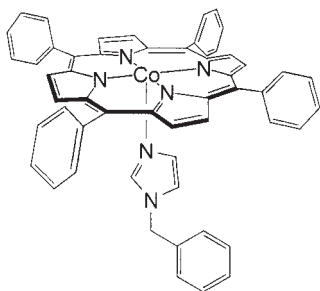
Chart 1. Tetraphenylporphyrinatocobalt(II)–benzylimidazole ([Co(tpp)(bim)]) complex.
